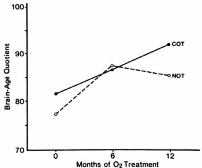
Fig. 12. Change in "fluid intelligence" (brain age quotient) in relation to continuous (COT) versus nocturnal (NOT) oxygen treatment in COPD patients. (From Reference 22, with permission.)
