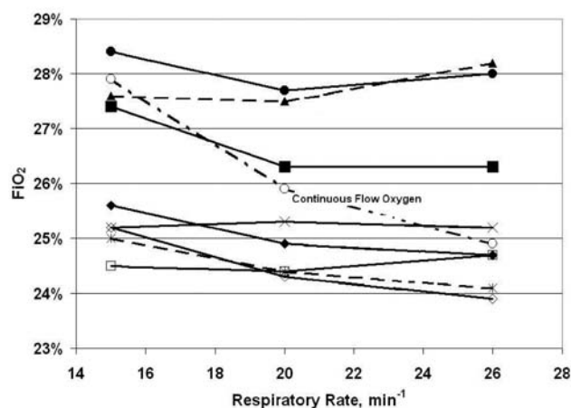
Figure 14. Graphic of eight conserving devices set at 2 L/min. With increased respiratory rate, FiO_2 varied between devices and continuous flow. Oxygen equivalency is a fallacy between continuous flow and different conserving devices.
